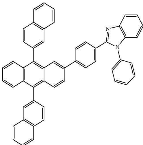
Compound 102
