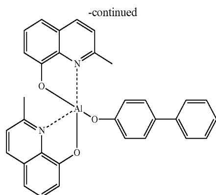
BAIq
